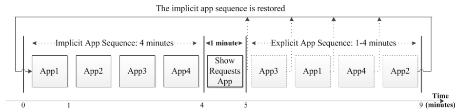
Figure 2: Applications presentation logic
